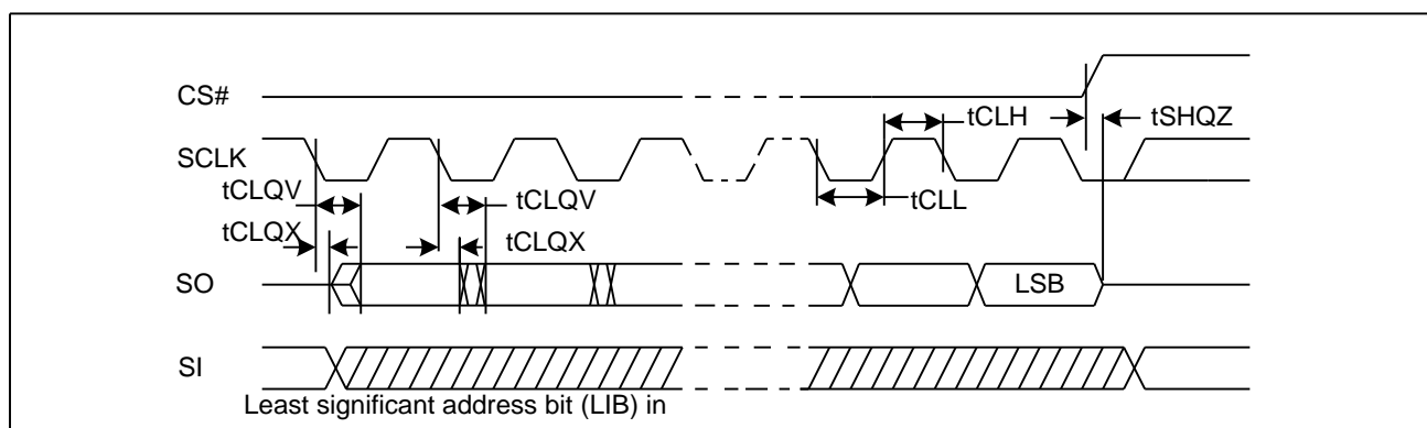
Figure 64. Output Timing
