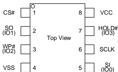
8 - LEAD SOP
