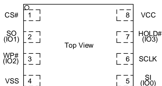
8 - LEAD USON/WSO
