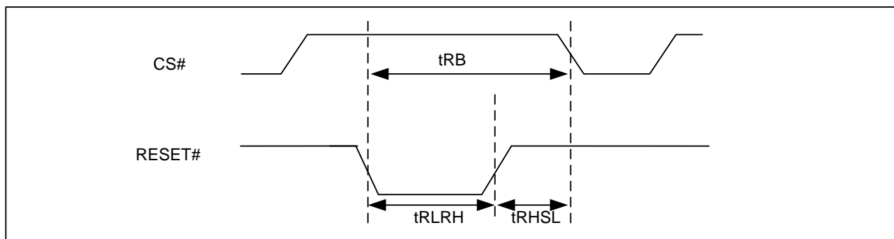
Figure 67 RESET Timing
