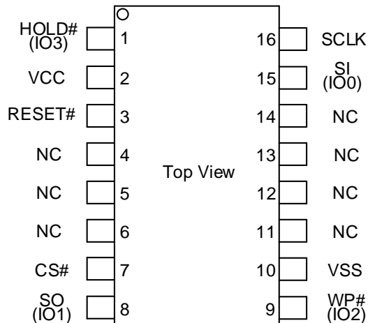
16-LEAD SOP
