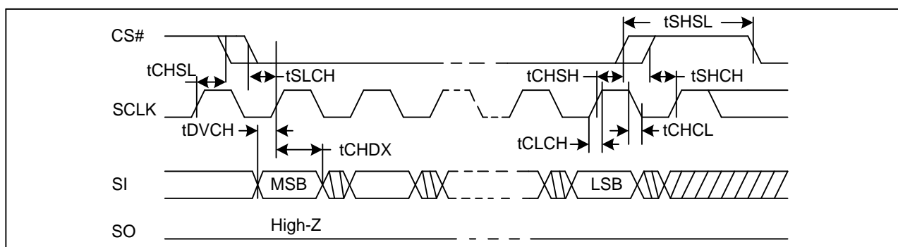
Figure 63. Input Timing
